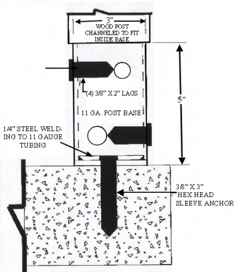
WOOD POST DETAIL
