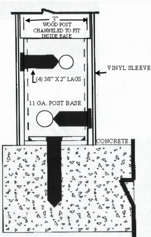
VINYL POST DETAIL
